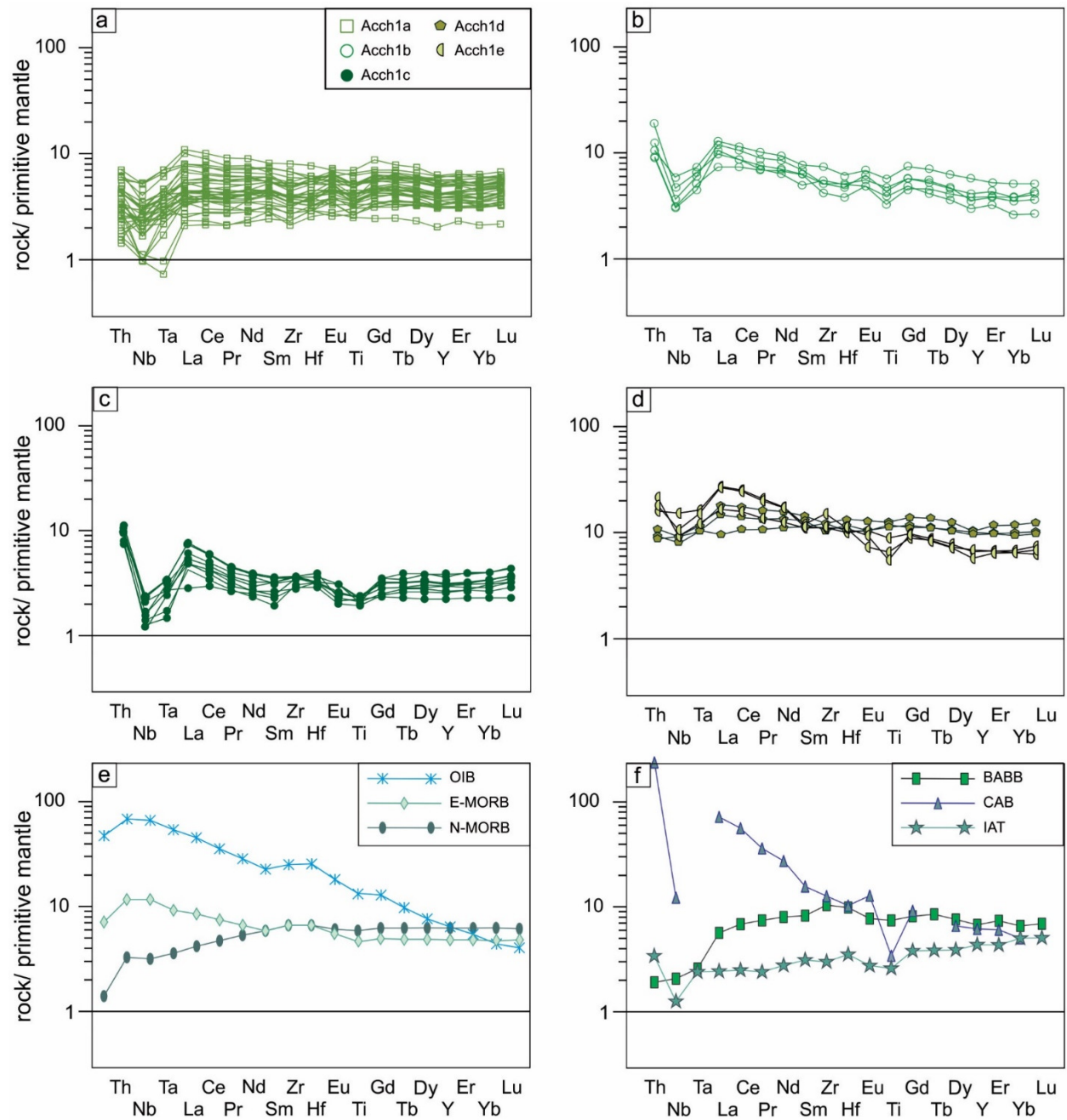
Fig. 7 Extended multi-element plots for the mafic lavas of the Colomb-Chaboullié greenstone belt. a) Acch1a , b) Acch1b , c) Acch1c , d) Acch1d and Acch1e , e) modern non-arc basalts, and f) modern arc basalts. Primitive mantle normalization values, normal mid-ocean ridge basalts (N-MORB), enriched mid-ocean ridge basalts (E-MORB), and ocean island basalts (OIB) are from Sun and McDonough (1989). The values for calc-alkaline basalts (CAB) and island arc tholeiites (IAT) are from Stolz et al. (1990), and for back-arc basin basalts (BABB) are from Ewart et al. (1994).
