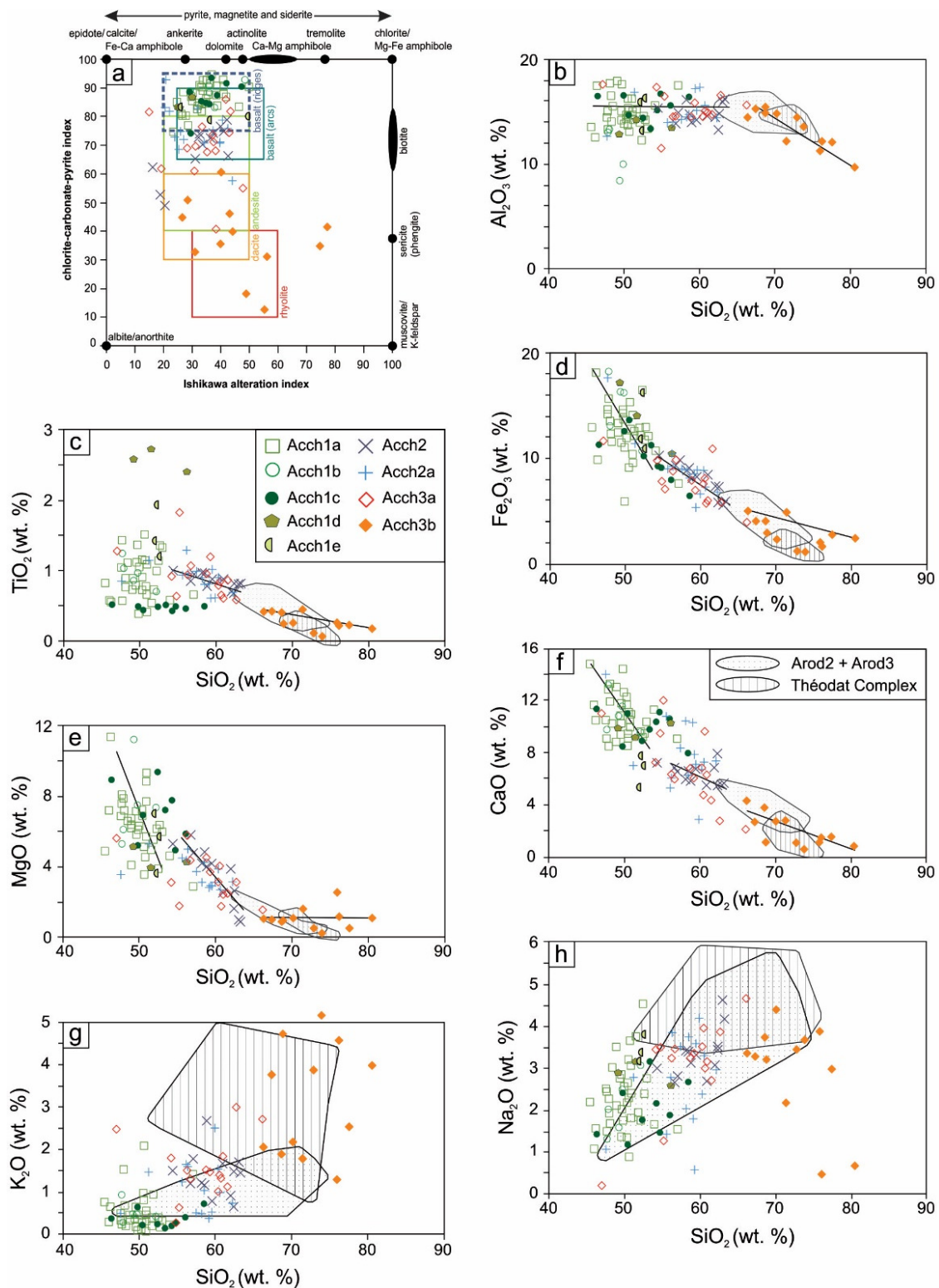
Fig. 5 Alteration box plot and Harker compositional diagrams for the Colomb-Chaboullié greenstone belt. (a) AI-CCPI alteration box plot (after Large et al., 2001). AI = 100(K_2O + MgO) / (K_2O + MgO + Na_2O + CaO) ; CCPI = 100(MgO + FeO^I) / (MgO + FeO^I + Na_2O + K_2O) . The box for unaltered ridge basalts on the alteration box plot is from Rogers et al. (2014) and the least altered boxes for arc basalts to rhyolites are derived from Gifkins et al. (2005). The poles for biotite and various amphiboles are from Caté et al. (2015). (b) - (h) SiO 2 versus Al 2 O 3 , TiO 2 , Fe 2 O 3 , MgO, CaO, K 2 O, and Na 2 O. Trend lines are included on the Harker diagrams in order to provide visual aid between the mafic, intermediate and felsic trends. Abbreviations: Arod2 + Arod3 : subunits of the Lac Rodayer pluton.
