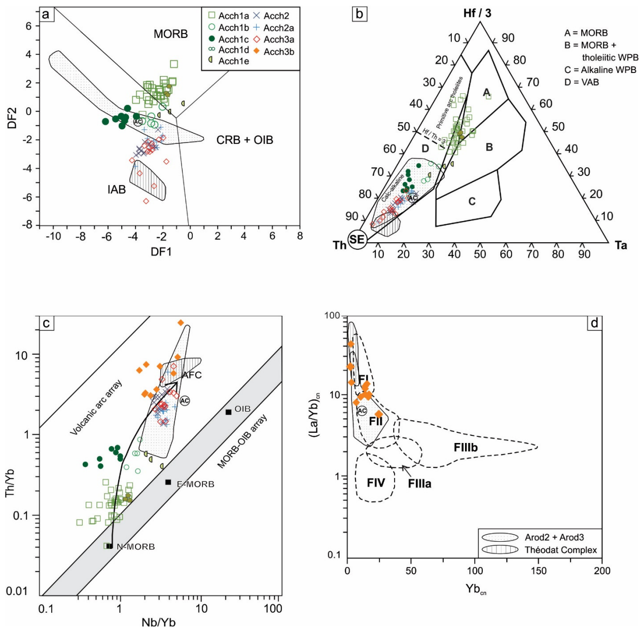
Fig. 8 Tectonic discrimination and rhyolite fertility diagrams. a) DF1-DF2 diagram of Agrawal et al. (2008). DF1 = 0.3518 \log_e(La/Th) + 0.6013 \log_e(Sm/Th) - 1.3450 \log_e(Yb/Th) + 2.1056 \log_e(Nb/Th) - 5.4763 ; DF2 = -0.3050 \log_e(La/Th) - 1.1801 \log_e(Sm/Th) + 1.6189 \log_e(Yb/Th) + 1.2260 \log_e(Nb/Th) - 0.9944 . IAB: island arc basalts; MORB: mid-ocean ridge basalts; CRB: continental rift basalts; OIB: ocean island basalts. b) Th-Hf-Ta ternary diagram from Wood (1980). The Archean crust (AC); after Rudnick and Fountain (1995) and subduction enrichment (SE) values are indicated. N-MORB: normal mid-ocean ridge basalts; E-MORB: enriched mid-ocean ridge basalts; WPB: within-plate basalts, VAB: volcanic arc basalts. c) Th/Yb vs. Nb/Yb diagram from Pearce (2008). AFC: assimilation-fractional crystallisation. d) (La/Yb)_{cn} versus Yb_{cn} after Hart et al. (2004). FI: alkali dacites and rhyodacites; FII: calc-alkaline rhyodacites and rhyolites; FIII: tholeiitic rhyolites; FIV: depleted rhyolites and high-silica rhyolites. Abbreviations; Arod2 + Arod3: subunits of the Lac Rodayer pluton.
