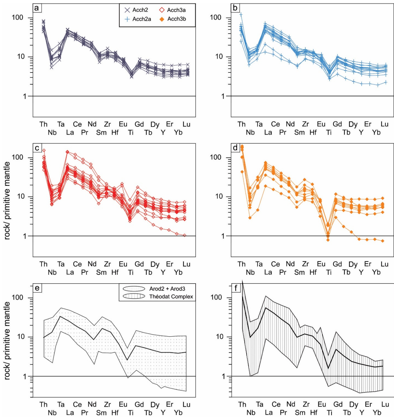
Fig. 9 Extended multi-element diagrams for the intermediate extrusive lavas, and intermediate to felsic volcanoclastic rocks of the Colomb-Chaboullié belt, as well as possible contaminants from the Opatica Subprovince. a) Acch2 , b) Acch2a , c) Acch3a , d) Acch3b , e) Arod2 + Arod3 , and f) Théodat Complex. Solid lines represent averages in (e)-(f). Primitive mantle normalisation values are from Sun and McDonough (1989). Abbreviations; Arod2 + Arod3 : subunits of the Lac Rodayer pluton.
